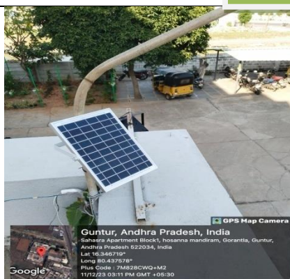
Solar portico lights-30vts
